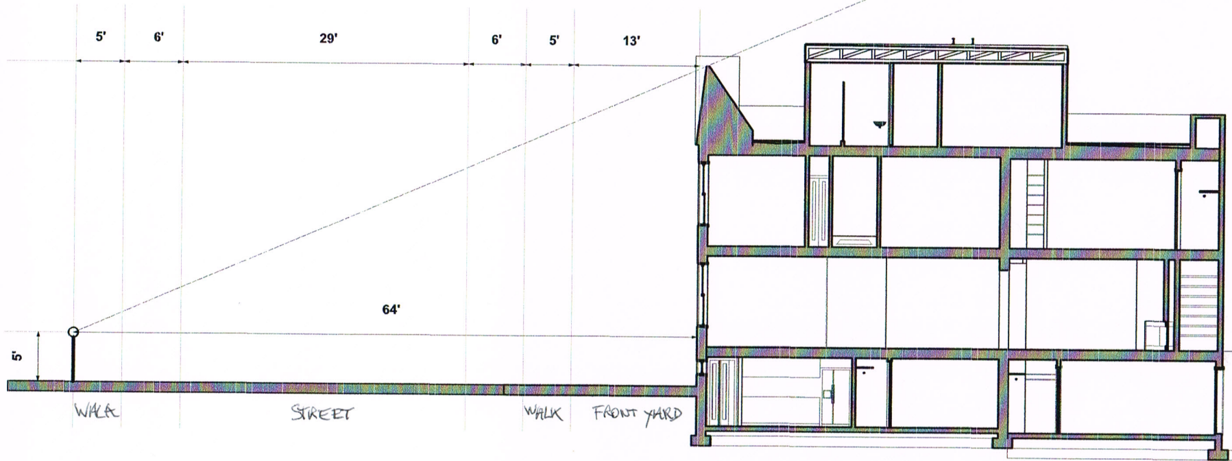
STREET PROFILE VIEW OF 1108 5TH STREET NE SHOWING LINE OF SITE ACROSS HIGHEST POINT OF BUILDING 1/4"=1'0"
